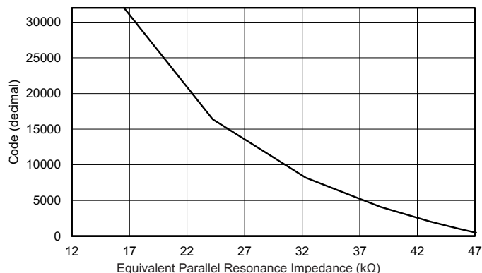
Figure 10. Transfer Characteristics of LDC1000-Q1 With R_{p\_MIN} = 16.160 \text{ k}\Omega and R_{p\_MAX} = 48.481 \text{ k}\Omega
